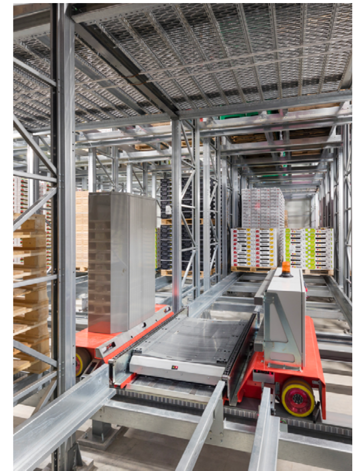
AUTOMATICO CON SATELLITE MOTHER-CHILD AUTOMATED STORAGE SYSTEM WITH MOTHER-CHILD SHUTTLE SYSTEM
